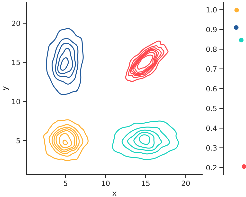
Joint distribution
