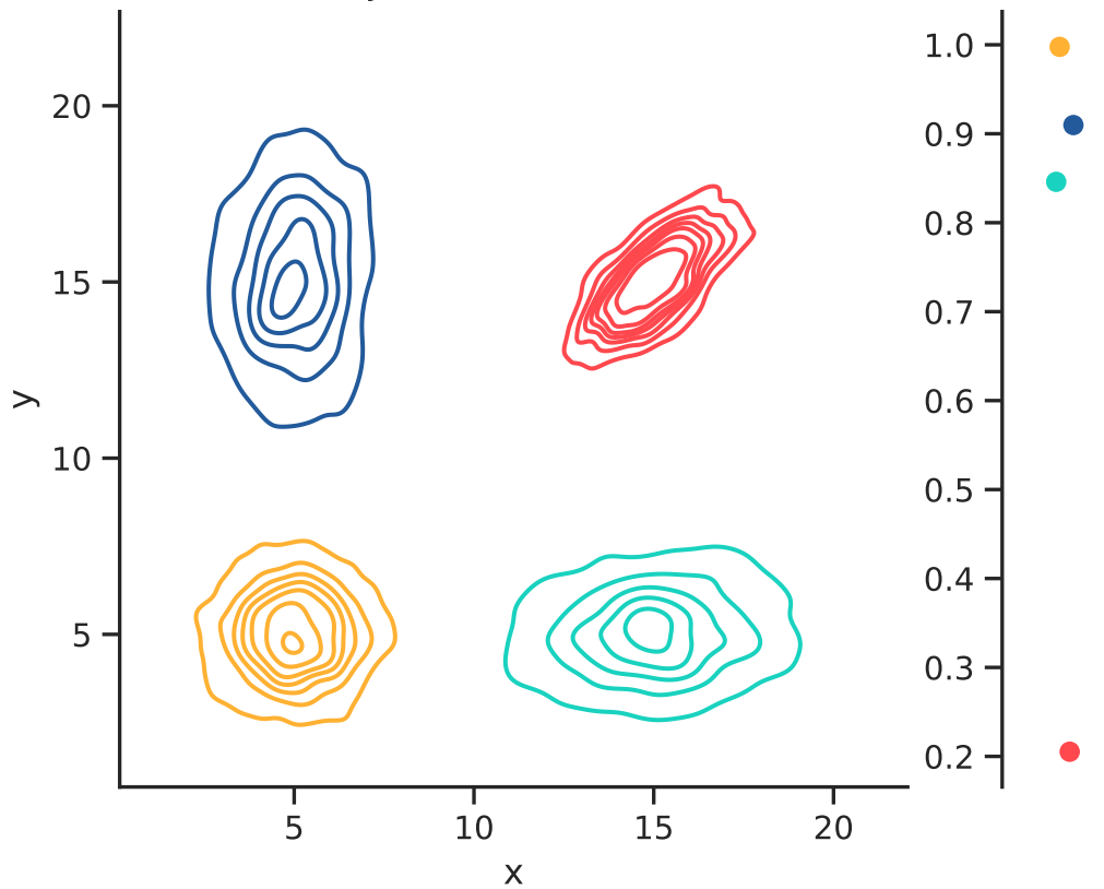
Joint distribution
