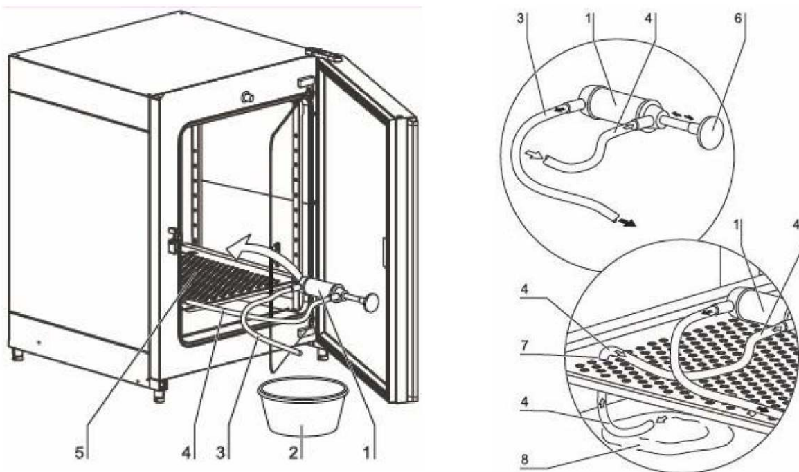
Fig. 5: Diagram of the water pump setup and parts: (1) pump, (2) bucket, (3) outlet hose, (4) inlet hose, (5) lowest incubator shelf, (6) pump hand grip, (7) incubator shelf hole, (8) water on incubator floor.
