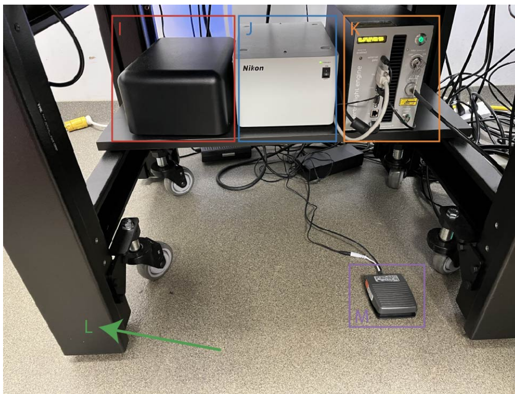
Fig. 6: I (red): Digital camera controller, J (blue): Microscope controller, K (orange): Epifluorescence light source, L (green): Air table (compressor not pictured), M (purple): Incubation chamber light switch
