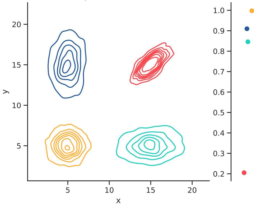
Joint distribution
